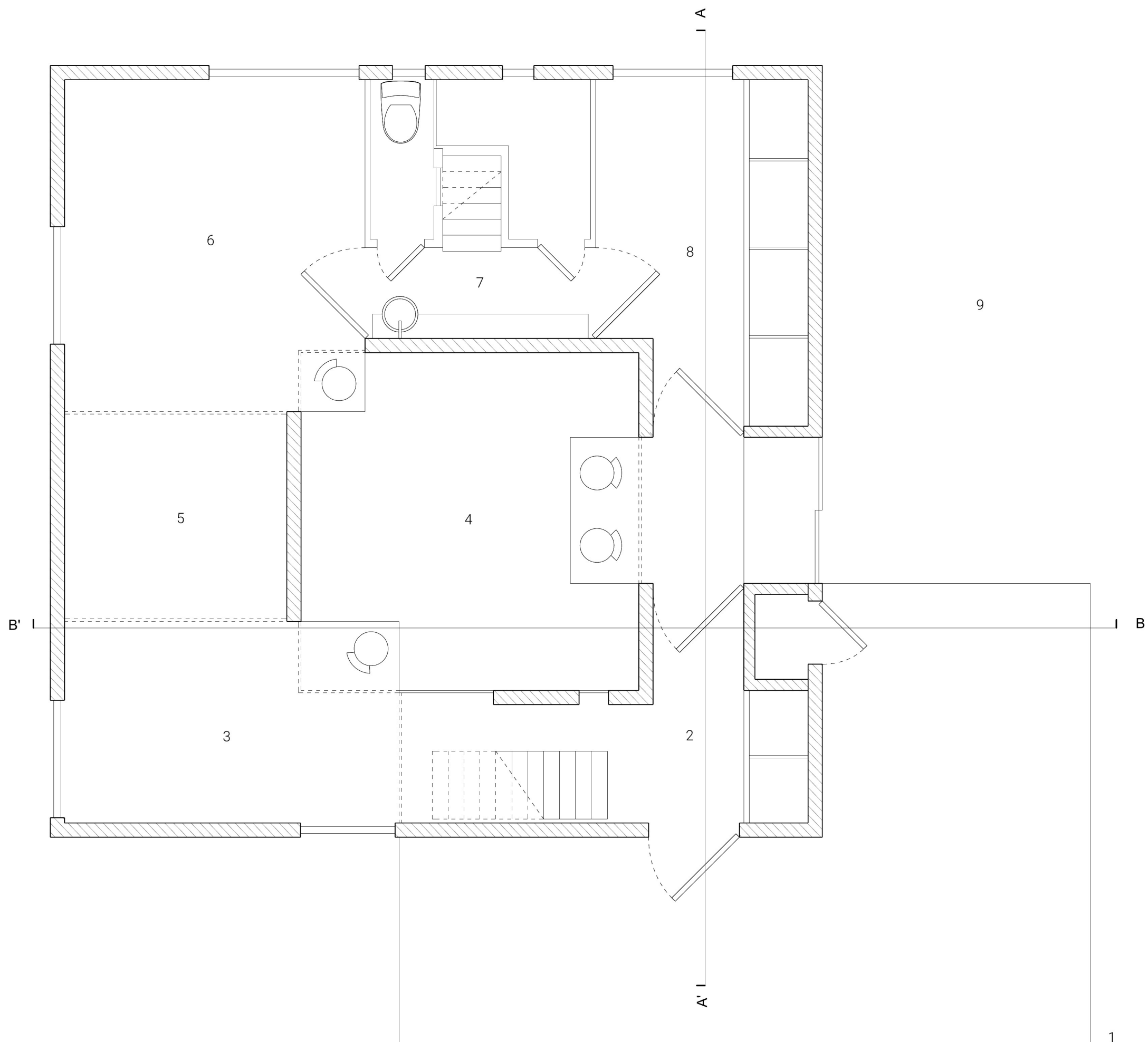
HOUSE IN SAKURADAI, GROUND FLOOR PLAN 1/8" = 1'-0"
